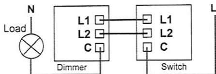
Figure 2. Using a 2-way Dimmerswitch.
