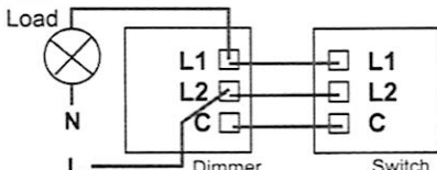
Figure 3. Using a 2-way Dimmerswitch.
