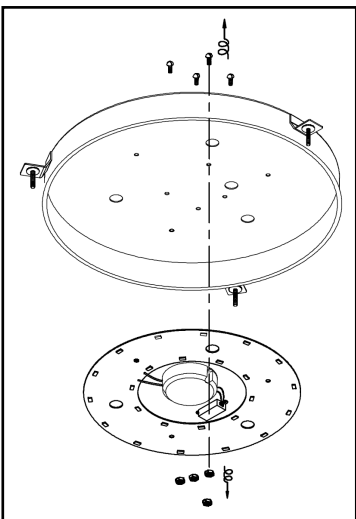
LED CHIP &amp; DRIVER REMOVAL
