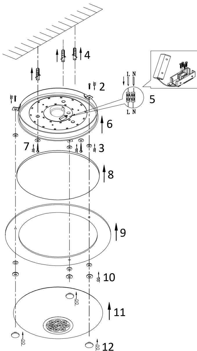
LED CHIP &amp; DRIVER REMOVAL
