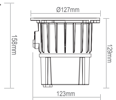
LED body
